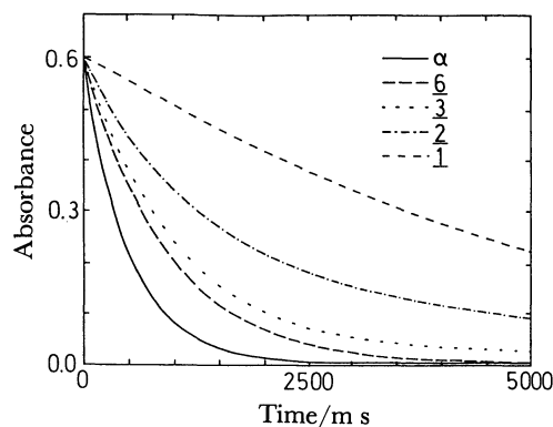
Fig. 2. The decay of phenoxyl radicals for the reaction of phenoxyls with tocopherol model compounds in ethanol at 25.0°C. [PhO \cdot ] 0 =0.05 mM and [Toc] 0 =0.50 mM. At 376 nm.
